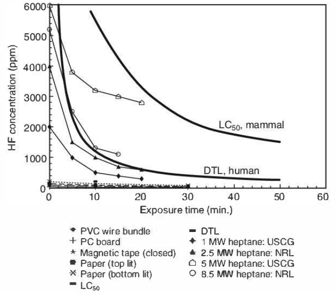
FIGURE A.7.5.1(b) Hazard Assessment of HF Concentrations. Extinguishment of Typical EDP and Class B Hazards with 7 Percent HFC-227ea.
