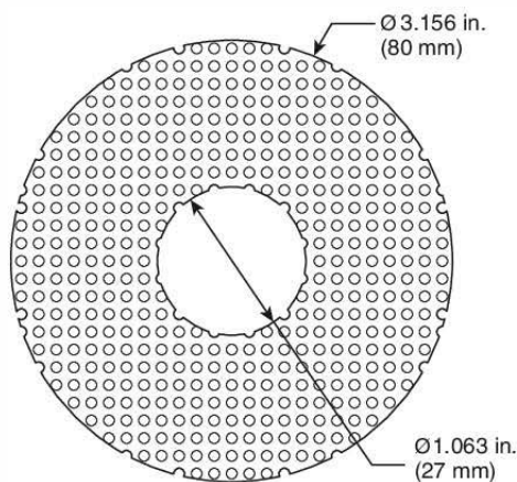
FIGURE C.17(f) Diffuser Bead Support Screen. (Material: 304 SS).
