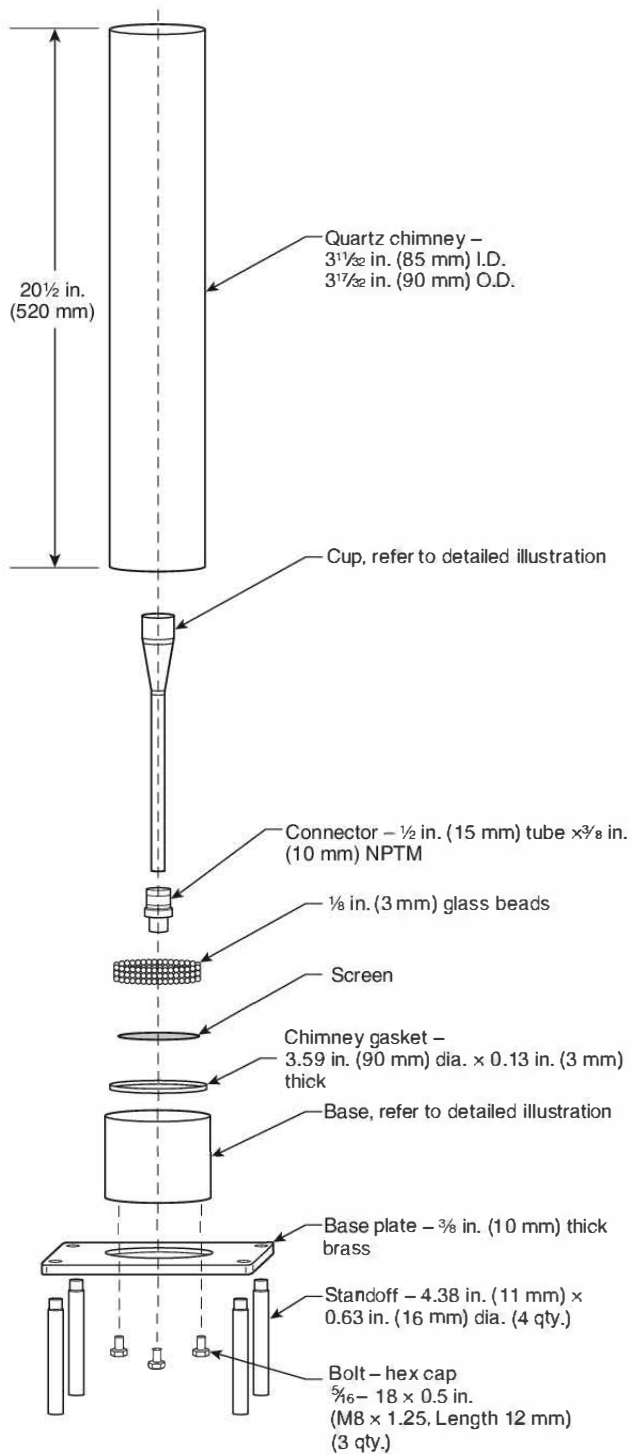
FIGURE C.17(a) Cup Burner Assembly (Exploded View).
