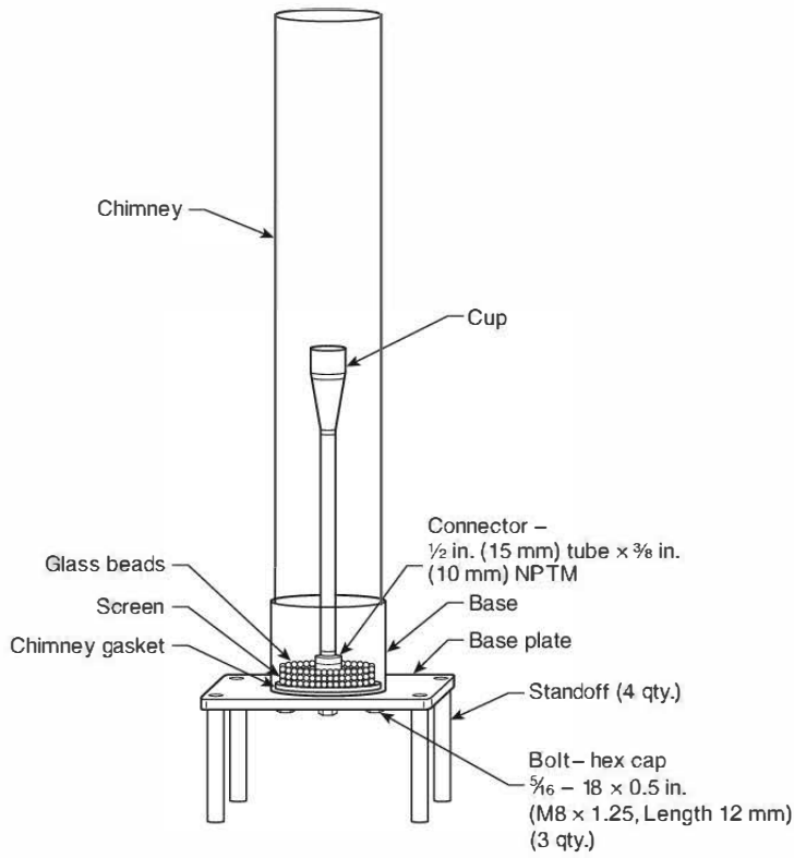
FIGURE C.17(b) Cup Burner Assembly (Transparent View).
