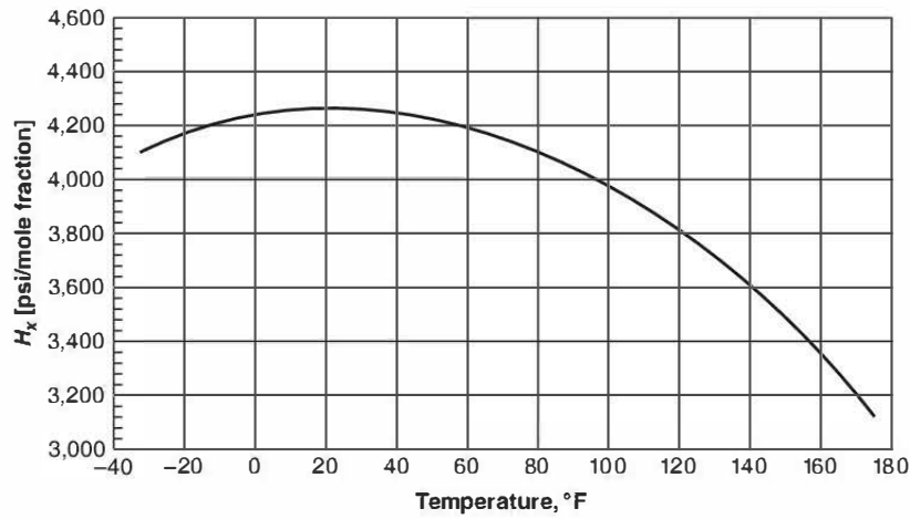
FIGURE F.2.2.2(a) HFC-227ea: Henry's Law Constant, H_x , for Nitrogen Solubility, US Units.
