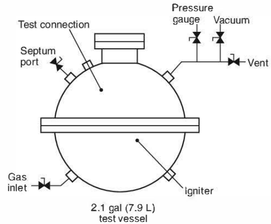
FIGURE A.7.2.3.1 Spherical Test Vessel.
