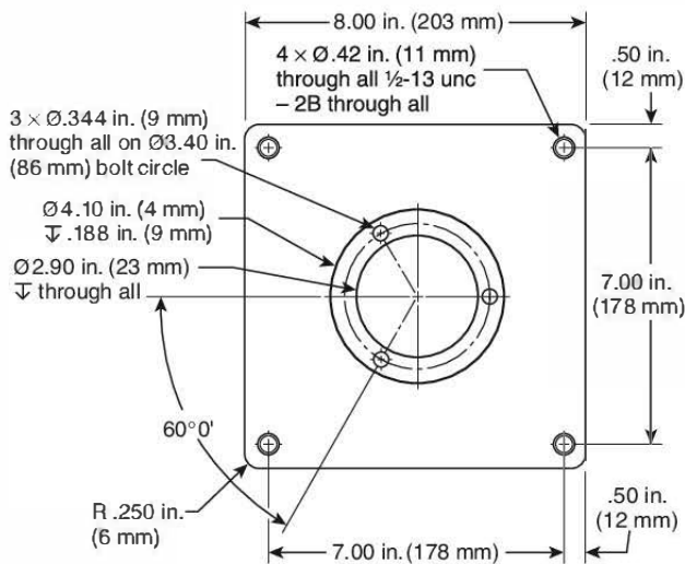
FIGURE C.17(e) Base Support Plate, \frac{3}{8} in. (10 mm) Thick.
