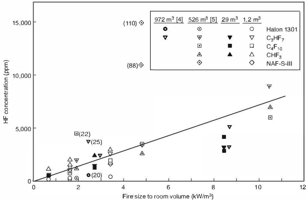
FIGURE A.7.5.1(a) Peak HF Concentrations.
