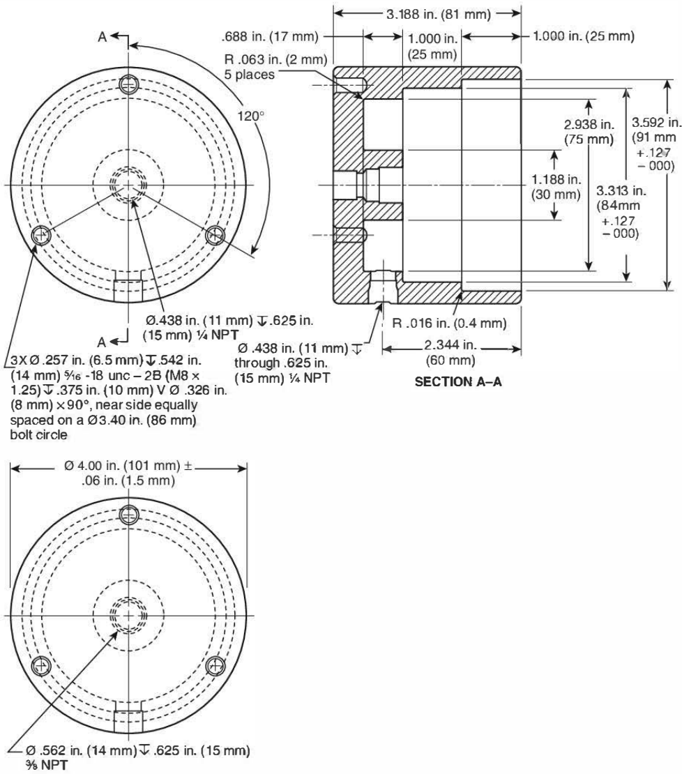
FIGURE C.17(d) Base, Detail.
