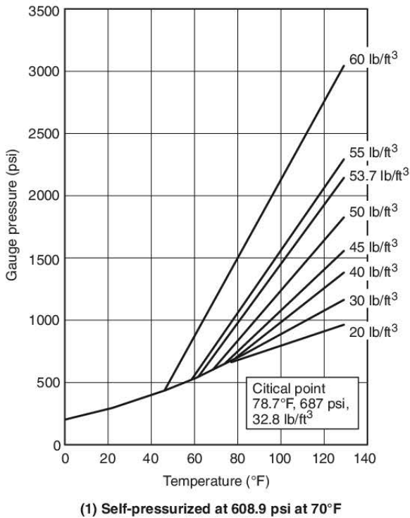
FIGURE A.5.1.4.1(g) Isometric Design of HFC-23.
